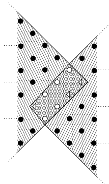
FIGURE 4. If it is known that the triangular nodes are in \text{Heap}(w) , then Lemma 1 tells us that all the white circles are also in \text{Heap}(w) .
