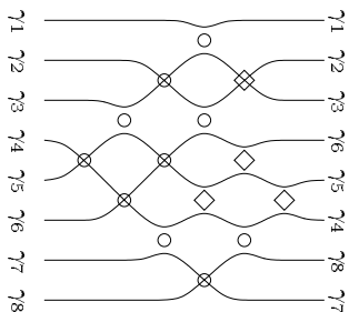
FIGURE 6. \text{Heap}(w) overlaid with a string diagram for the reduced expression \mathbf{a} = s_4s_3s_2s_1s_5s_4s_3s_2s_6s_5s_4s_7s_6s_5 and \boldsymbol{\sigma} = (1, 0, 1, 0, 1, 1, 0, 0, 0, 1, 0, 0) . Note that \pi(w^\boldsymbol{\sigma}) = s_4s_5s_4s_7 , giving the permutation [1, 2, 3, 6, 5, 4, 8, 7] . The defects are represented by diamonds. As an illustration of our terminology regarding strings, note that \gamma_{47} meet at \text{pt}(9) (for our reduced expression \mathbf{a} ). And \gamma_6 encounters \text{pt}(j) for j \in \{5, 6, 7, 11\} (also for \mathbf{a} ).
