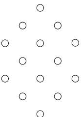
FIGURE 2. \text{Heap}(u) for u as in (8).
