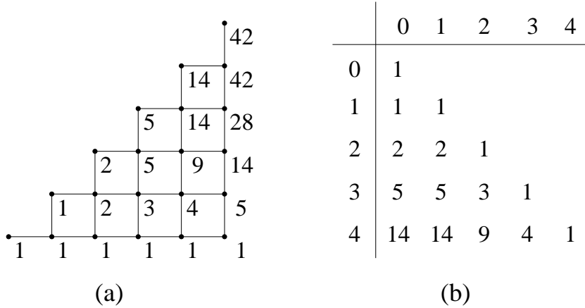
Figure 1: Representations for Dyck paths.
