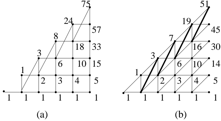
Figure 2: Two schemes illustrating privileged access to the main diagonal.
