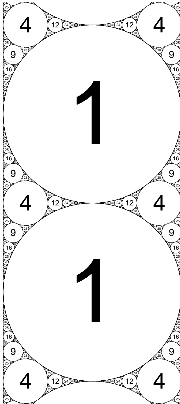
Figure 2: The Apollonian circle packing (0, 0, 1, 1) .
