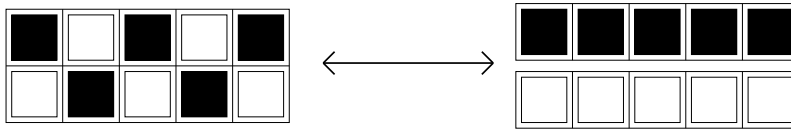
Figure 4: Finding M_{2,5} .
