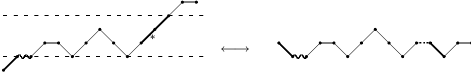
Figure 3: Elevation of a partial 2-Motzkin path
