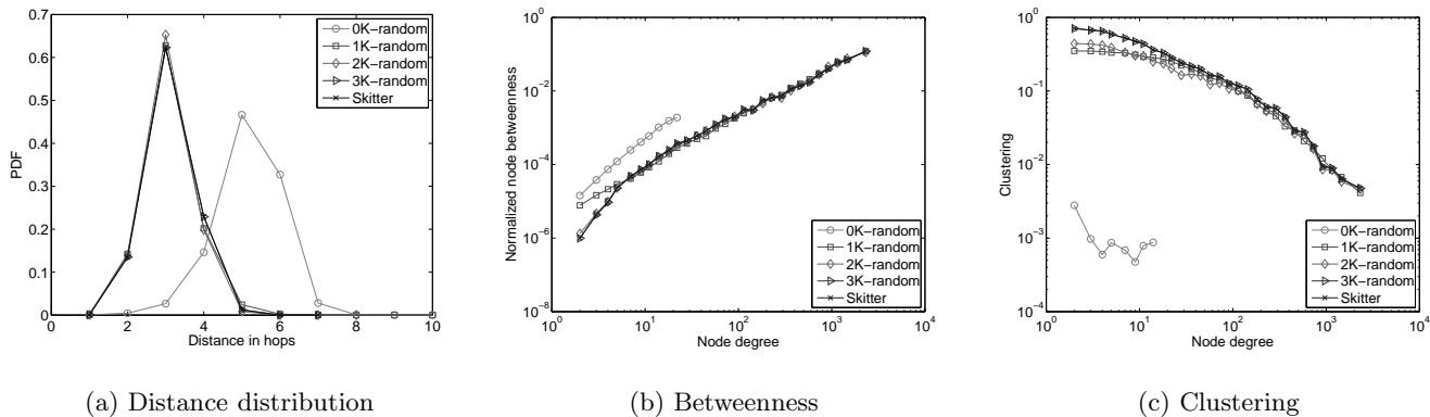
Figure 6: Comparison of dK -random and skitter graphs.
