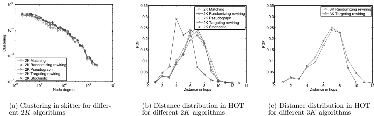
Figure 5: Comparison of 2K- and 3K-graph-constructing algorithms.
