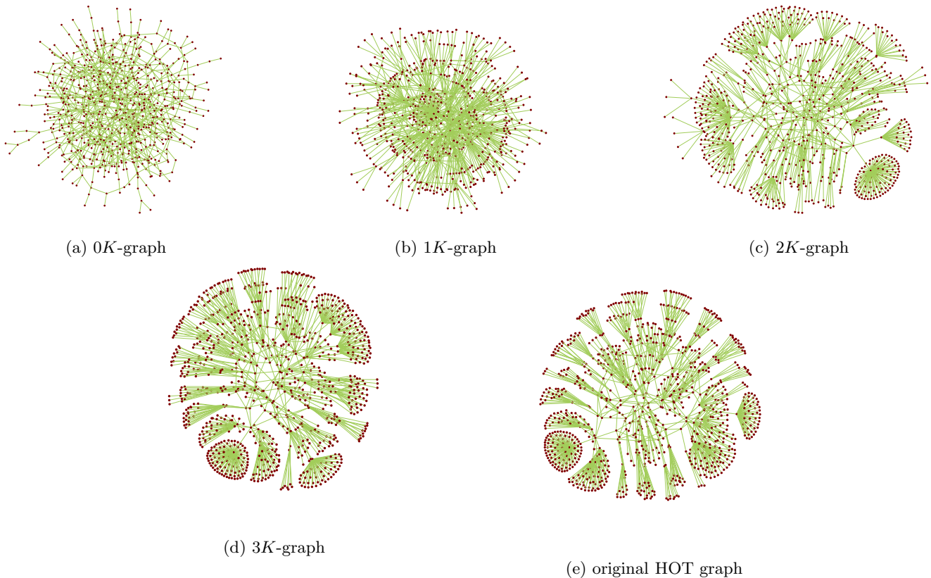
Figure 3: Picturizations of dK -graphs and the original HOT graph illustrating the convergence of dK -series.
