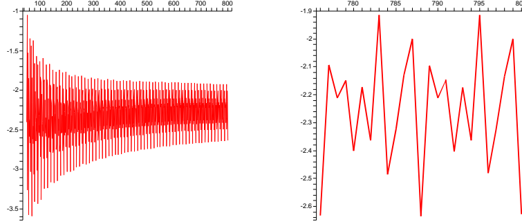
FIGURE 2. Permutations with distinct cycle lengths: the approximation error as measured by n^4 \log^3 n (f_n / (\widehat{f}_n^{[1]} + \widehat{f}_n^{[-1]} + \widehat{f}_n^{[\omega]} + \widehat{f}_n^{[\omega^2]}) - 1) , with the \widehat{f}_n truncated after n^{-3} terms, for n = 50 \dots 800 (left) and for n = 776 \dots 800 (right).
