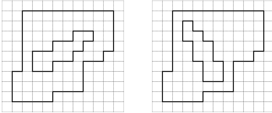
Figure 1. The left panel shows a typical punctured staircase polygon and the right panel a rotated punctured staircase polygon.
