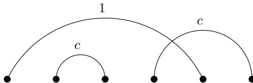
FIGURE 1.3. The same complete matching under the rightmost-choice weighting, in which edges with no right crossing have weight c and others have weight 1. This is used in the orthogonality proof.
