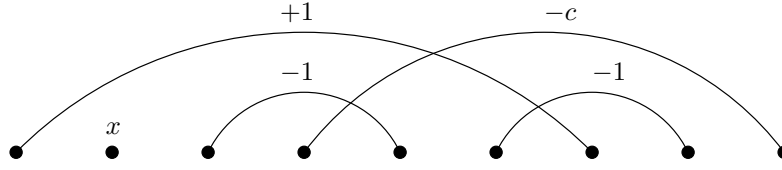
FIGURE 4.4. A matching on 9 vertices that contributes cx to H_7(x; c + 1) using the combinatorial interpretation of Theorem 4.6 . Note the “fake edge” of weight +1 .
