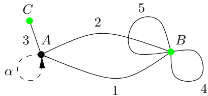
FIGURE 4.1. A rooted map to which we'll apply the bijection to connected matchings. Green vertices have weight c . We have already added the extra edge, labeled \alpha ; the original root was the end of edge 1 incident with vertex A .
