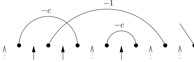
FIGURE 4.3. A matching on 6 vertices of the type described by Lemma 4.4. If the new edge on the right is to have weight -1 and satisfy the conditions, it must connect to a new vertex in one of the three available slots, indicated by the solid arrows.
