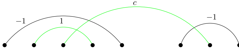
FIGURE 1.4. A paired matching for n = 5 and m = 3 .
