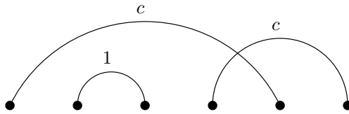
FIGURE 1.2. A complete matching on 6 points under the leftmost-choice weighting for the moments, in which nonnested edges have weight c and others have weight 1.
