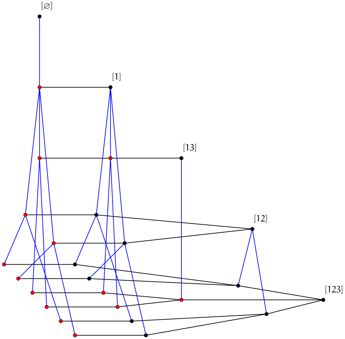
FIGURE 4. The rooted twofold forest for type A_3 .
