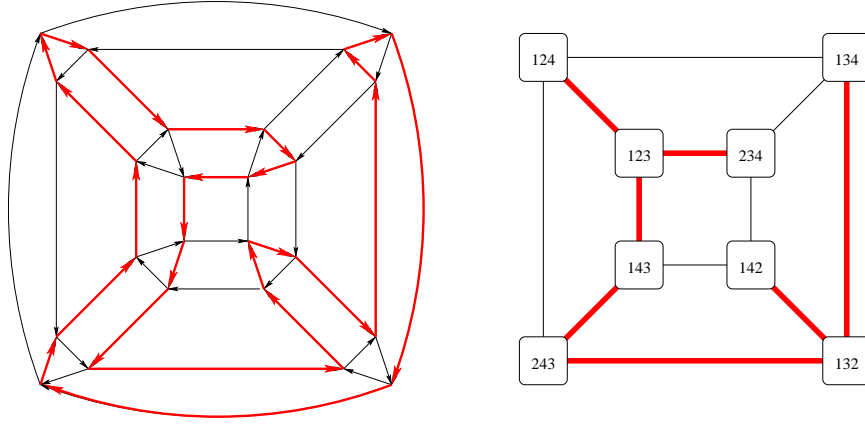
FIGURE 1. The Cayley graph \Xi_4 on the left. The graph Q_4 on the right. The thick (red) edges indicate the Hamiltonian cycle S_4 .
