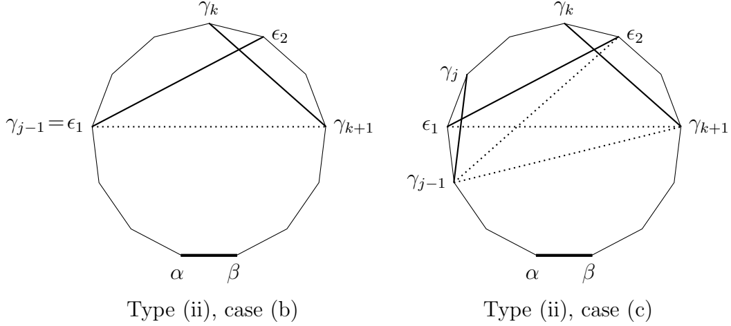
FIGURE 5. In type (ii), the diagonal \{\epsilon_1, \epsilon_2\} forces the presence of the diagonal \{\gamma_{j-1}, \gamma_{k+1}\} .
