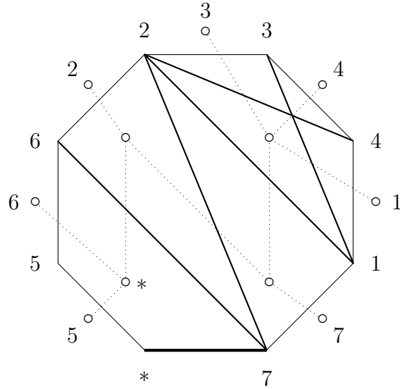
FIGURE 7. The correspondence between R' -enriched rooted trees and labelled Ptolemy diagrams with base edge.
