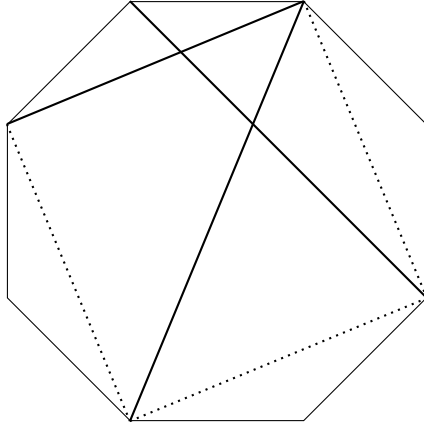
FIGURE 3. The dotted diagonals are \text{nc} of the solid diagonals
