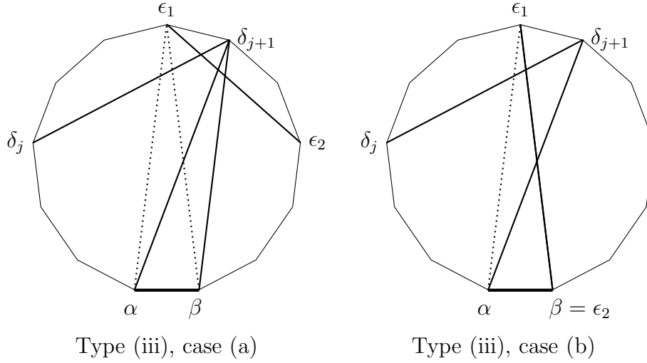
FIGURE 6. In type (iii), the diagonal \{\epsilon_1, \epsilon_2\} forces the presence of the diagonals \{\alpha, \epsilon_1\} and \{\beta, \epsilon_1\} .
