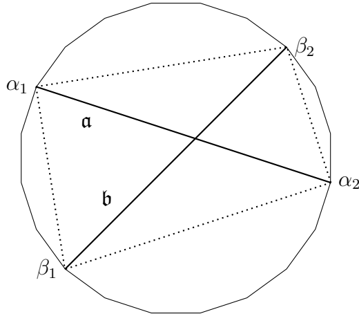
FIGURE 1. The Ptolemy condition
