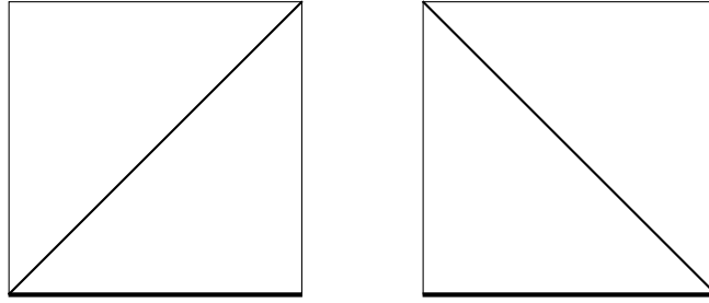
FIGURE 2. Two different Ptolemy diagrams
