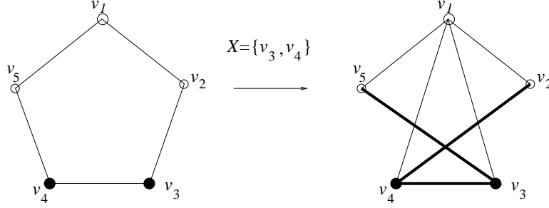
FIGURE 2. The action with X = \{v_3, v_4\}
