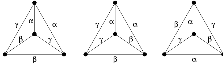
FIGURE 5. The first weight corresponds to a zero of \tau_W , but the second two do not.
