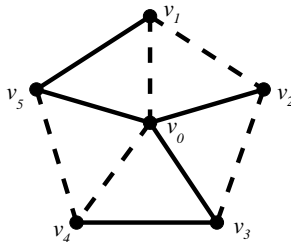
FIGURE 1. Two complementary coupled spanning trees of a 5-wheel
