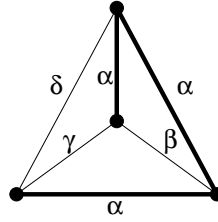
FIGURE 4. A weight induced P_4
