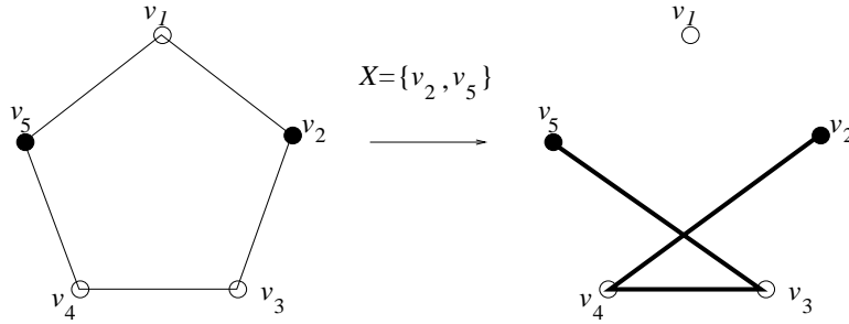
FIGURE 3. The action with X = \{v_2, v_5\}
