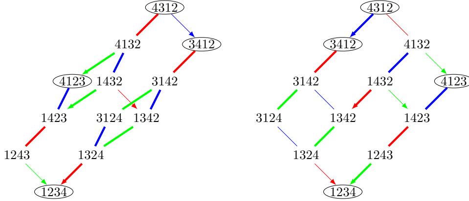
FIGURE 1. Two pictures of the interval [1234, 4312]_R in \mathfrak{S}_4 illustrating its proper tilings, for J := \{3\} and J := \{1, 2\} , respectively. The thick edges highlight the tiling. The circled permutations are the cutting points, which are at the top of the tiling intervals. Blue, red, green lines correspond to s_1, s_2, s_3 , respectively. See Section 6.4 for the definition of the orientation of the edges (this is G^{(4312)} ); edges with no arrow tips point in both directions.
