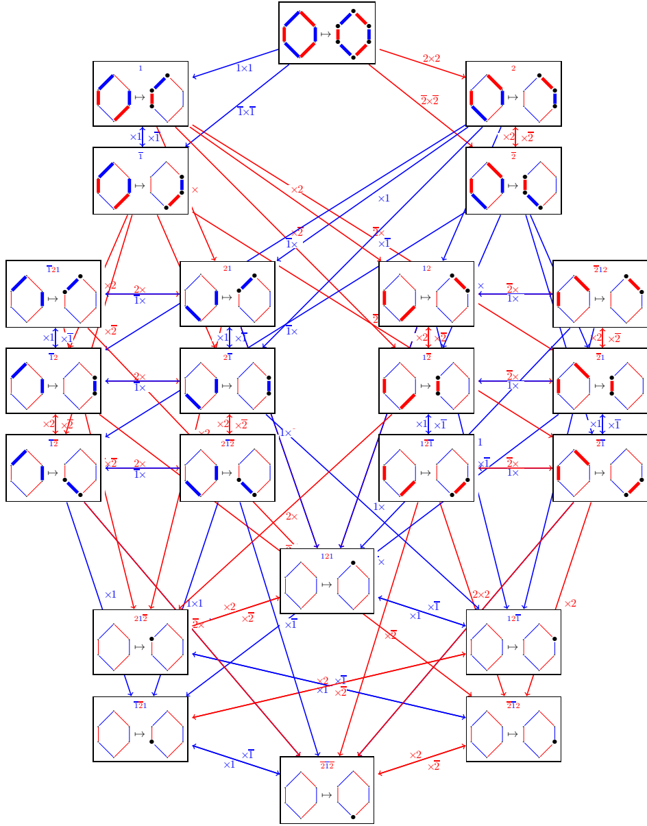
FIGURE 5. The graph of \mathcal{J} -order for M(\mathfrak{S}_3) . The vertices are the 23 elements of M(\mathfrak{S}_3) , each drawn as in Figure 4. The edges give both the left and right Cayley graph of M(\mathfrak{S}_3) ; for example, there is an arrow f \xrightarrow{\times \pi_1} g if g = f\pi_1 , and an arrow f \xrightarrow{\pi_1 \times \pi_1} g if g = f\pi_1 = \pi_1 f . The picture also highlights the \mathcal{J} -classes of M(\mathfrak{S}_3) , and the corresponding eggbox pictures (i.e. the decomposition of the \mathcal{J} -classes into \mathcal{L} and \mathcal{R} -classes); namely, from top to bottom, there is one \mathcal{J} -class of size 1 = 1 \times 1 , two \mathcal{J} -classes of size 2 = 1 \times 2 , two \mathcal{J} -classes of size 6 = 2 \times 3 , and one \mathcal{J} -class of size 6 = 1 \times 6 , where n \times m gives the dimension of the eggbox picture. In other words the \mathcal{J} -class splits into n \mathcal{R} -classes of size m and also into m \mathcal{L} -classes of size n . This example is specific in that all \mathcal{J} -classes are regular.
