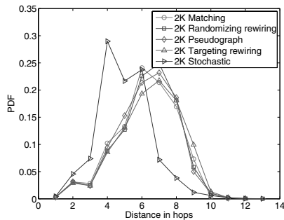
(b) Distance distribution in HOT for different 2K algorithms
