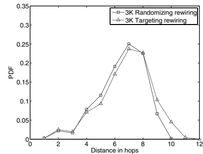
(c) Distance distribution in HOT for different 3K algorithms
