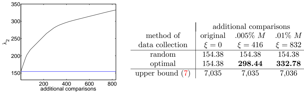
Figure 5: (left) The informativeness of the ranking, \lambda_2(w) , as a small number ( .01\% \cdot M ) of targeted pairwise comparisons (black) and randomly selected pairwise comparisons (blue) are added. (right) The value of \lambda_2(w) for this augmented dataset and the upper bound on \lambda_2 given in (7). The change in informativeness for randomly added data is unappreciable compared to a 2.2 fold increase for targeted data. See §5.3.
