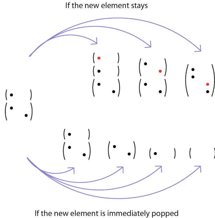
Figure 5: Example of possible transitions from a given r-state
