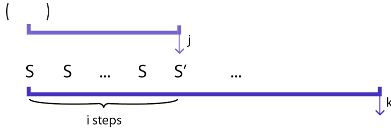
Figure 7: Example of signal passing in the case where the nonempty r-twinstack S changes after i steps for some integer i less than m
