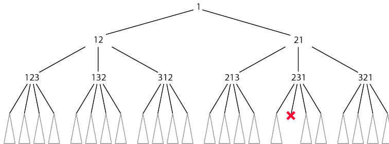
Figure 3: Searching the permutation tree
