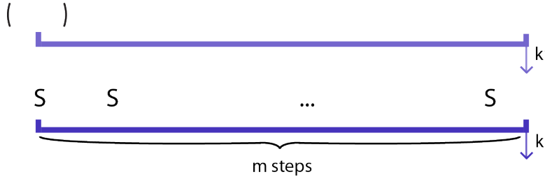
Figure 8: Example of signal passing in the case where the nonempty r-twinstack S remains unchanged up till the end of the epoch
