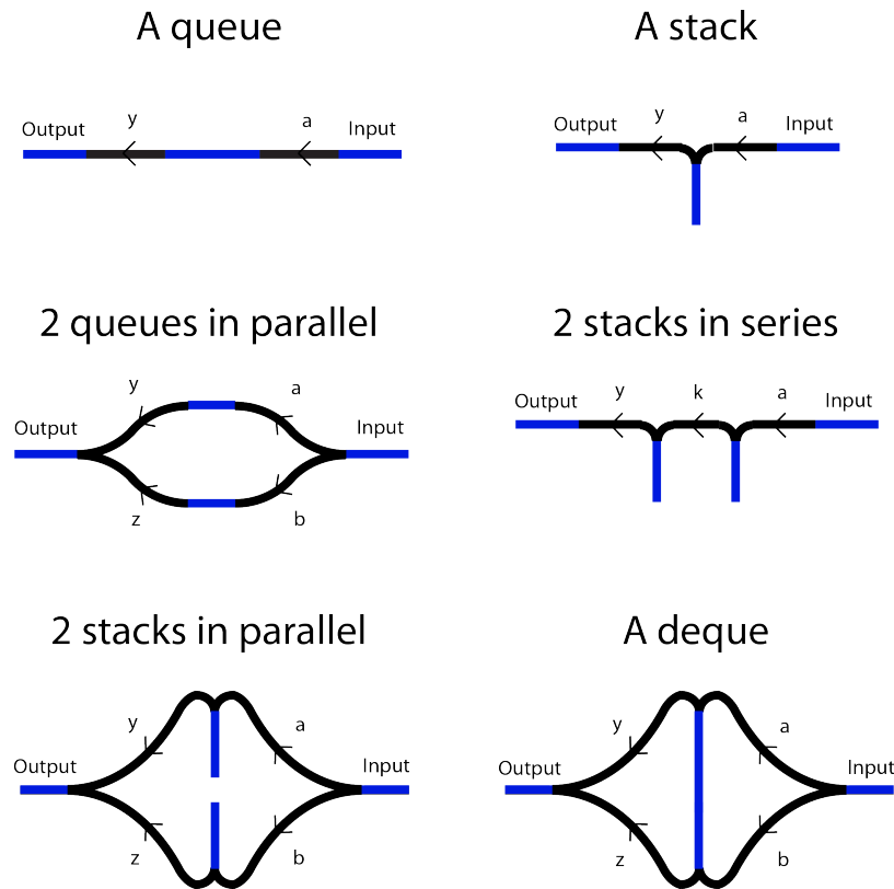
Figure 1: Some small switchyards
