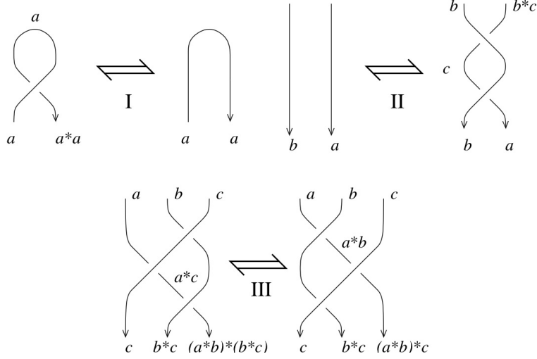
Figure 1: Reidemeister moves and the quandle identities
