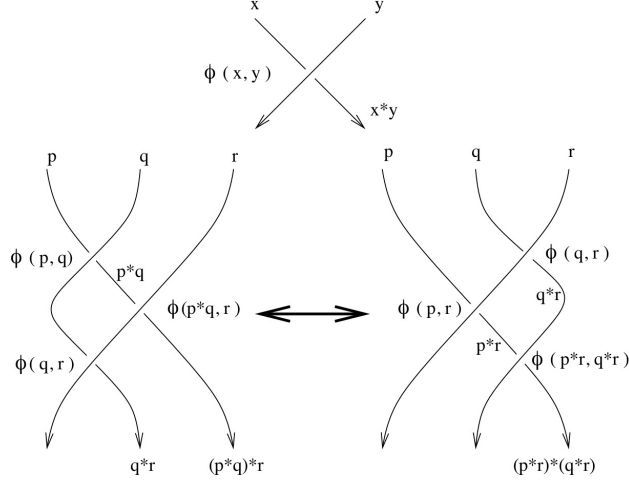
Figure 2: 2-cocycle condition coming from Type III move
