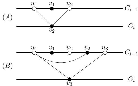
FIGURE 9. The two-valent vertex v_1 in C_{i-1} producing another two-valent vertex in C_i .
