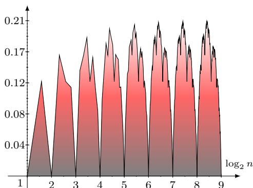
FIG 4. \frac{1}{2} \log_2 n - \mathbb{E}(X_n) .
