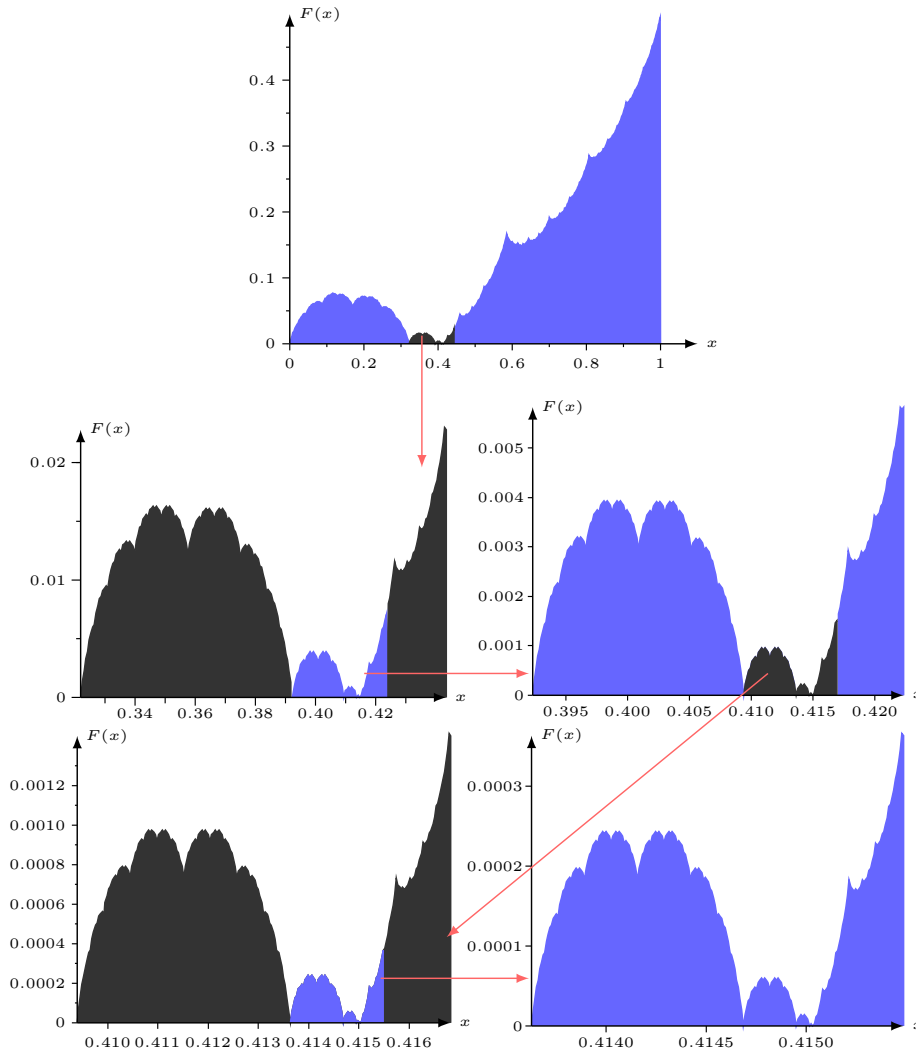
FIG 10. The fractal nature of the function |F(x)| .
