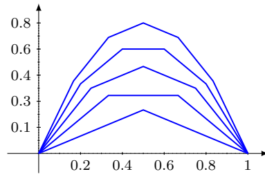
FIG 6. h(x) : q = \frac{6}{2} .
