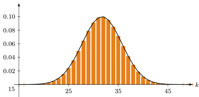
FIG 9. The histogram of X_{31415926535897932384} , where the black smooth curve represents the density with the same mean and the same variance.
