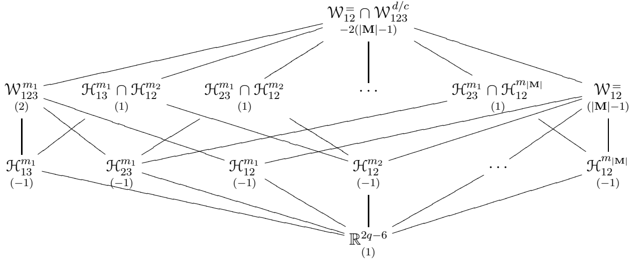
FIGURE 3.1. The computation of \mu(\hat{0}, W_{12}^{\bar{=}} \cap W_{123}^{d/c}) , exhibited in the Hasse diagram of the interval [\hat{0}, W_{12}^{\bar{=}} \cap W_{123}^{d/c}] in \mathcal{L}(\mathcal{A}_{\mathbb{P}}) , with the value of \mu(\hat{0}, \mathcal{U}) below the subspace \mathcal{U} . We let m_1 = d/c .
