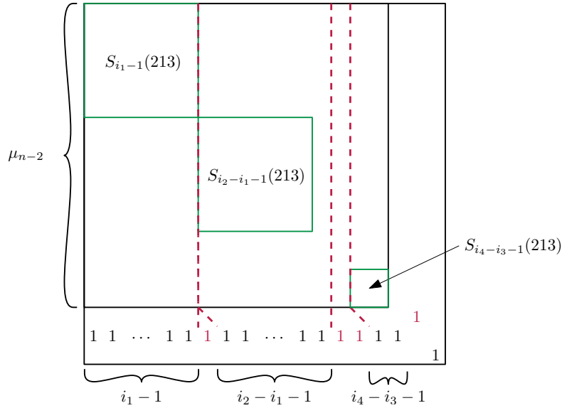
Figure 5: A partial embedding of the red elements, showing where the remaining blocks can be fit into the columns of \mu_{n-2} . The run of length 2 in the bottom right of the chessboard has been expanded for clarity.
