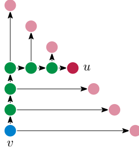
Figure 13: Example of the augmentation in Lemma 38. Immediate real descendants are colored red and the new fictitious nodes are colored green.
