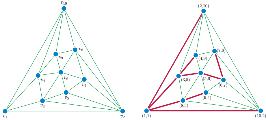
Figure 2: Left: a maximally planar graph G with canonically ordered vertices. Right: \text{ctree}(G) is shown in red, and the label around each vertex v indicates \text{pre}(v) and \text{post}(v) .
