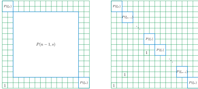
Figure 14: Chessboard representation of the superpattern P(n, s) . Each P(\xi_i) in the figure is P(\xi_i, s - 1) , with the s - 1 omitted because of space constraints.
