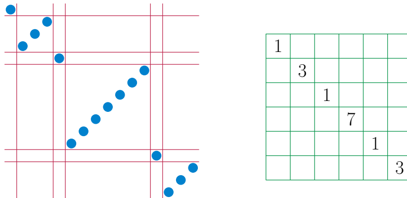
Figure 7: The S_7(213, 132) -superpattern
