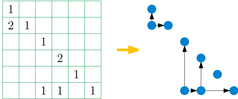
Figure 8: The chessboard of a permutation and its corresponding chessboard graph.
