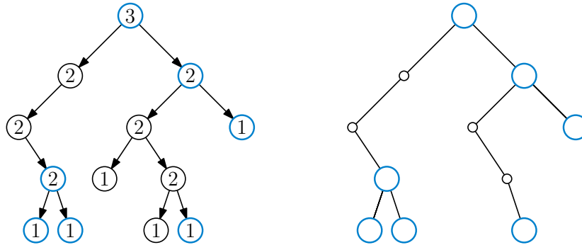
Figure 12: A tree with nodes labeled by their Strahler number and one of the underlying complete binary trees.
