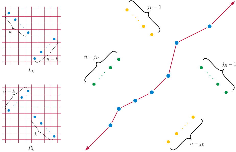
Figure 10: Left: The permutations we use to prove our lower bound for S_n(213, 132, 3412, 4231) -superpatterns. Right: The three sets of points we describe in the proof are shown respectively in blue, yellow, and green. The spine is shown in red.
