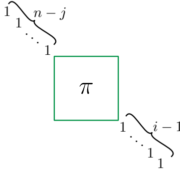
Figure 3: The permutation \tau constructed from \pi in the proof of Lemma 24
