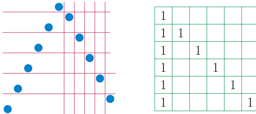
Figure 6: The S_6(213, 312) -superpattern
