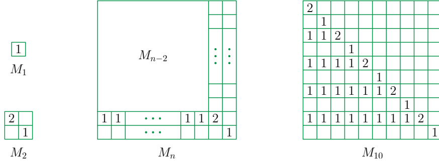
Figure 4: The base cases, \text{chessboard}(\mu_i) for i = 1, 2 , and the inductive construction of \text{chessboard}(\mu_n) from \text{chessboard}(\mu_{n-2}) . Cells of the matrices containing zero are shown as blank.
