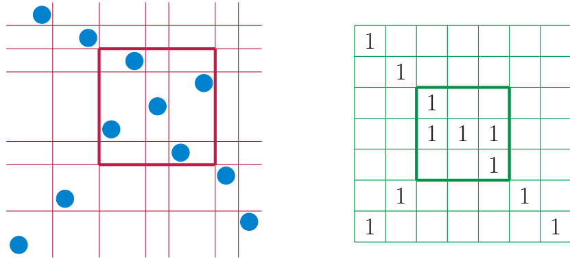
Figure 9: The S_5(213, 3412) -superpattern. The pattern inside the bolded box is the base case S_3 -superpattern.
