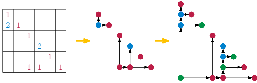
Figure 11: The chessboard of a permutation, its corresponding chessboard graph, and its tree augmentation from Lemma 33. Real vertices are colored red and blue, and fictitious vertices are colored green.
