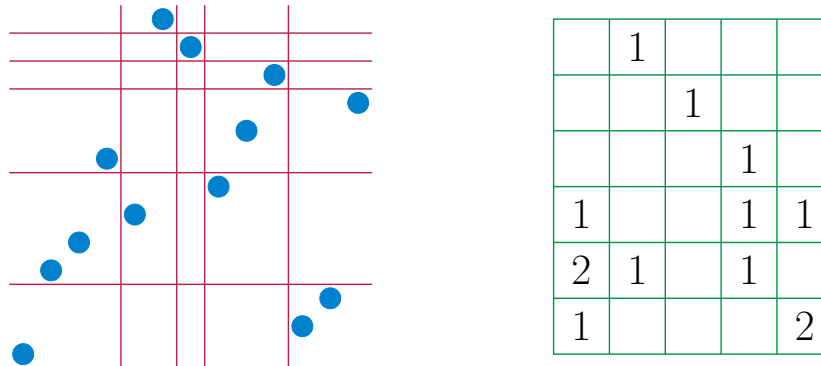
Figure 1: The permutation \pi = 1 4 5 8 6 13 12 7 9 11 2 3 10 represented by its scatterplot (the points (i, \pi_i) ) with lines separating its rows and columns (left), and by \text{chessboard}(\pi) (right).
