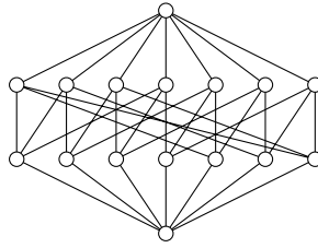
FIGURE 3. The subspace lattice of the Fano plane.
