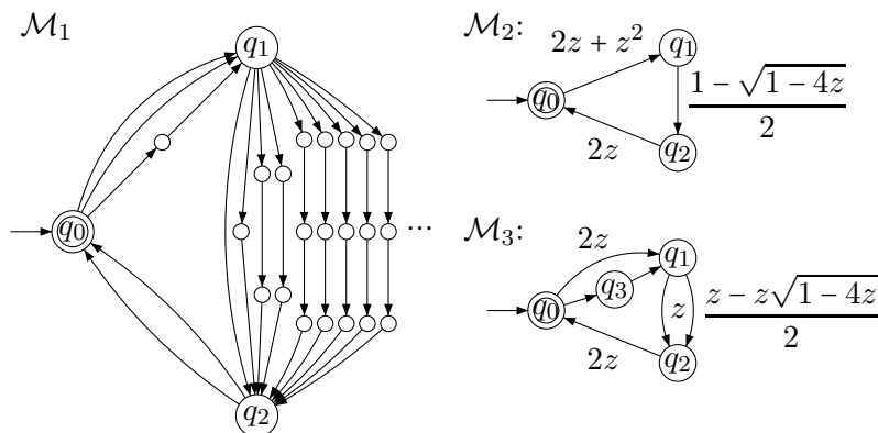
FIGURE 8. Counting automata with transitions in parallel, Example 11.
