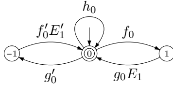
FIGURE 15. Equivalent automaton to \mathcal{M}_{\text{BLin}} .
