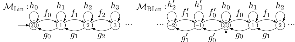
FIGURE 14. Infinite counting automata \mathcal{M}_{Lin} and \mathcal{M}_{BLin} .
