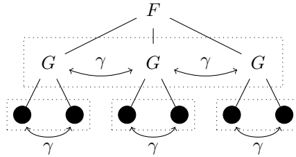
FIGURE 5. A schematic of an (F \circ G) -structure with an action of \gamma \in \Gamma
