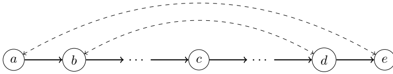
FIGURE 6. Schematic of a permutation (dashed arrows) which reverses a linear order (solid arrows)
