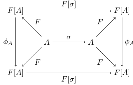
FIGURE 2. Diagram which must commute if \phi is a species automorphism
