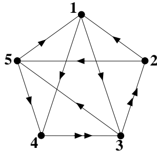
Figure 5: The Somos-5 quiver.
