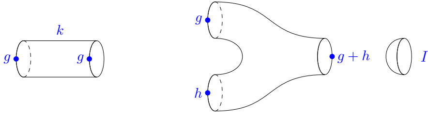
Figure 2: Elementary components of cobordisms: cylinder, pair of pants and disc.
