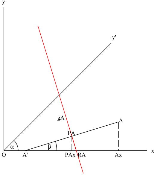
Figure 5: Folding A onto A'
