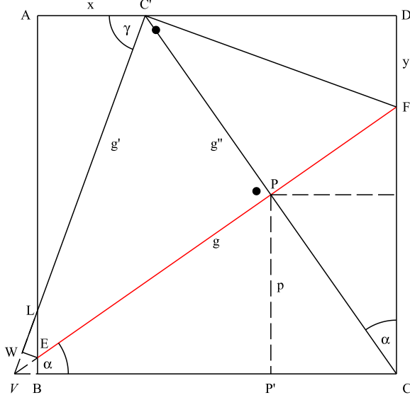
Figure 1: Folding C onto C'
