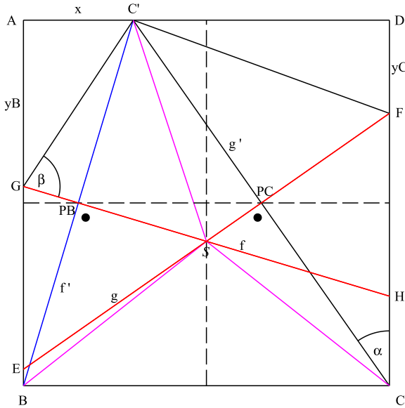
Figure 3: Folding C and B onto C' = B'
