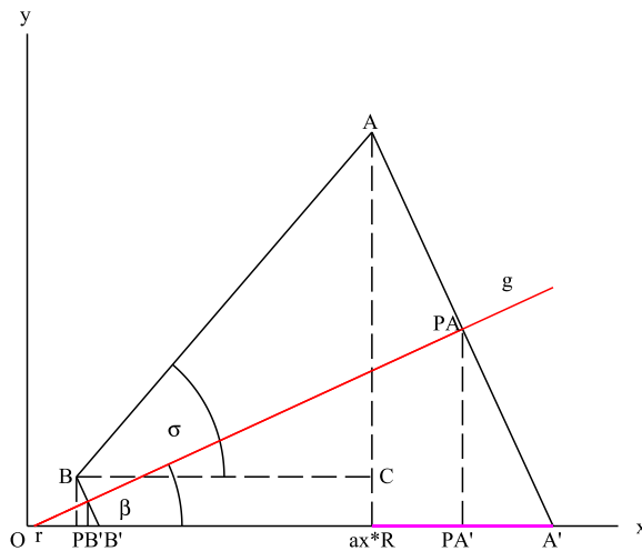
Figure 10: Folding A on A' and B on B' when \alpha = 0
