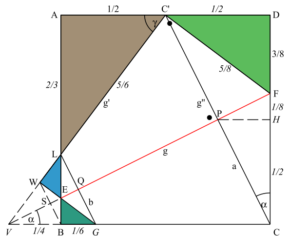
Figure 4: Haga's triple of Egyptian triangles
