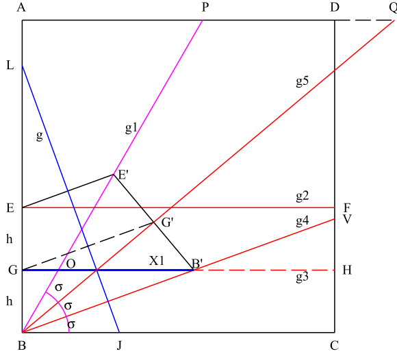
Figure 21: Solution X1: Trisecting an angle \alpha \alpha = 60^\circ and h = .2
