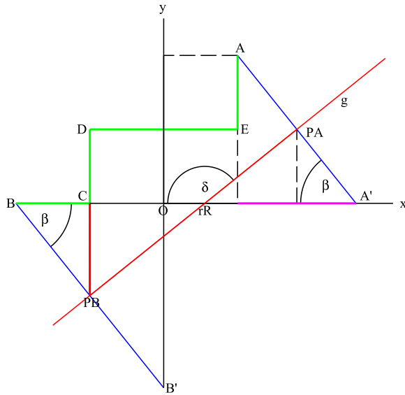
Figure 15: \alpha = \frac{\pi}{2} , heptagon, third origami
