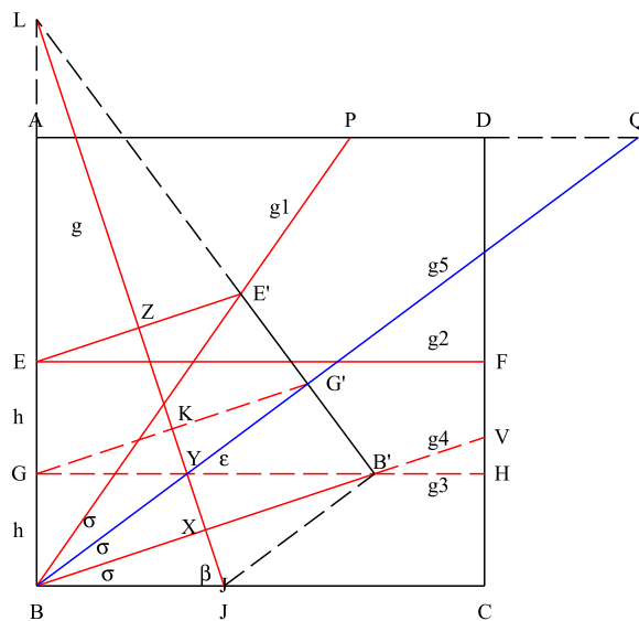
Figure 20: Trisecting an angle \alpha = 55^\circ and h = 0.25
