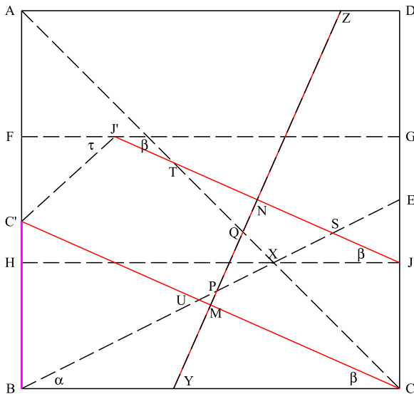
Figure 16: Doubling the cube; finding \overline{C', B}
