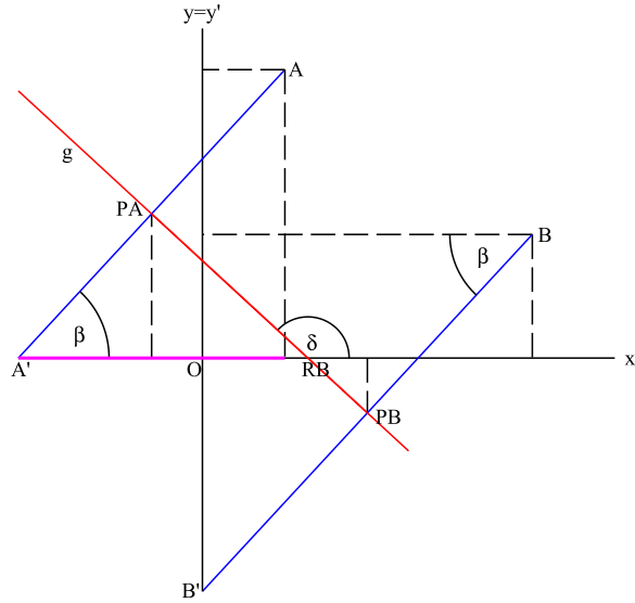
Figure 9: Folding A onto A' and B onto B'
