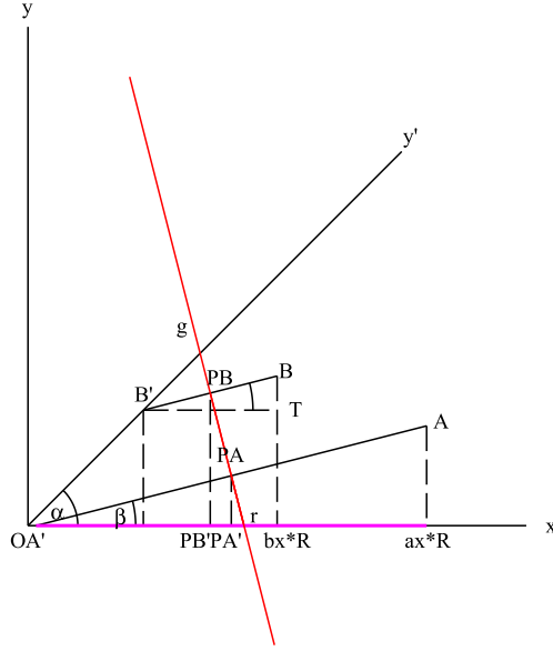
Figure 7: Third order eq. Folding A onto A' , and B onto B' , \alpha = 45^\circ
