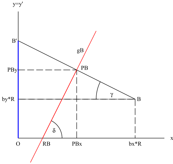
Figure 8: Folding B onto B'
