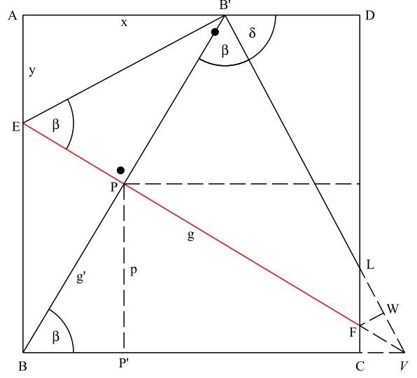
Figure 2: Folding B onto B'
