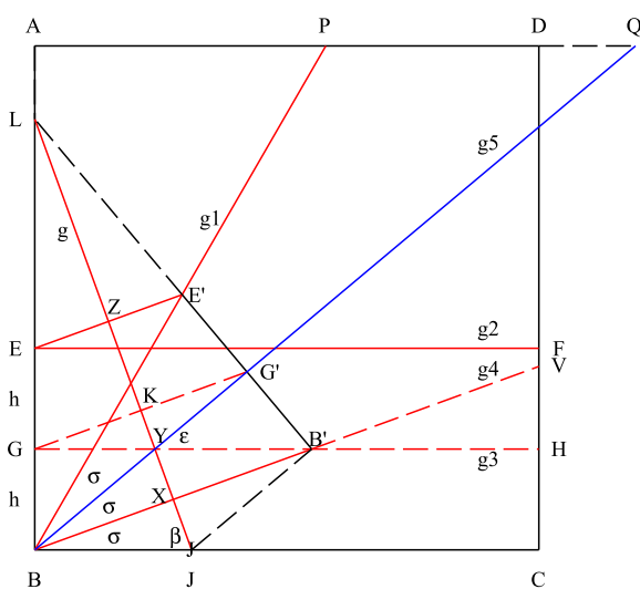
Figure 19: Trisecting an angle \alpha = 60^\circ and h = 0.2
