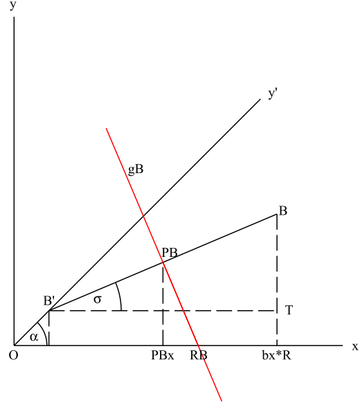
Figure 6: Folding B onto B'
