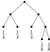
FIGURE 2.1. The canonical tree associated with the partition 1 = 3 \cdot 2^{-2} + 2 \cdot 2^{-3} of 1 into powers of 2. This partition has weight \frac{1}{12} and corresponds to 10 distinct compositions.
