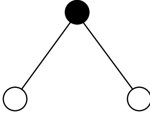
Figure 1: The ghost-free interaction terms present in DDG represented in a theory diagram. The absence of interaction terms mixing more than two dreibeine demands the diagram to be a graph. The absence of ghosts further requires the graph to be a tree and the lines between the nodes represent the two invertible linear combinations of dreibeine, as in (22). In addition, the dreibein which couples to the other two dreibeine should have an inverse, denoted as a solid circle.
