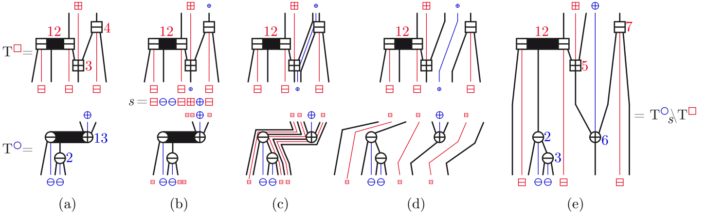
FIGURE 43. (a) Two Schröder-Cambrian trees \mathbf{T}^{\circ} and \mathbf{T}^{\square} . (b) Given the shuffle s = \square \circ \square \circ \square \square \circ \square \square , the positions of the \square are reported in \mathbf{T}^{\circ} and the positions of the \circ are reported in \mathbf{T}^{\square} . (c) The corresponding laminations. (d) The trees are split according to the laminations. (e) The resulting Schröder-Cambrian tree \mathbf{T}^{\circ} \circ_s \mathbf{T}^{\square} .
