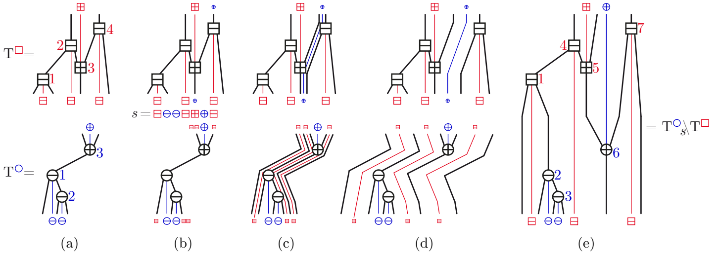
FIGURE 14. (a) The two Cambrian trees T^{\circ} and T^{\square} . (b) Given the shuffle s = \ominus \oplus \ominus \oplus \oplus \oplus \ominus , the positions of the \ominus are reported in T^{\circ} and the positions of the \oplus are reported in T^{\square} . (c) The corresponding laminations. (d) The trees are split according to the laminations. (e) The resulting Cambrian tree T^{\circledast}_s .
