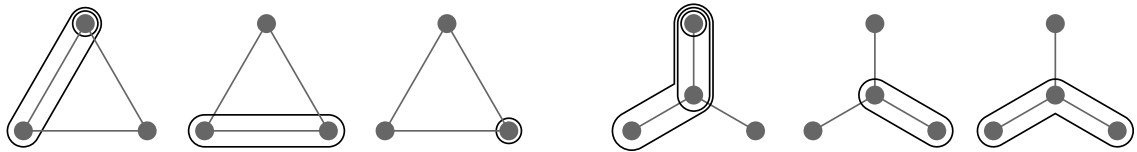
FIGURE 11. Counter-examples to the naive definition of compatibility degrees: both on the triangle and on the tripod, all tubes of the initial maximal tubing on the left are incompatible with the two distinct tubes on the right.
