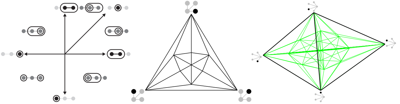
FIGURE 17. The compatibility fans \mathcal{D}(X_{n+1}, \mathbb{T}^\circ) for the star X_{n+1} and the initial tubing \mathbb{T}^\circ = \{\{\ell_1\}, \dots, \{\ell_n\}\} formed by its leaves (for n \in \{2, 3, 4\} ).
