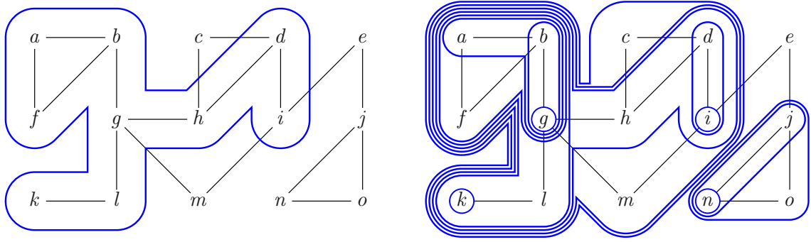
FIGURE 4. A tube \mathfrak{t}_{\text{ex}}^{\circ} of G_{\text{ex}} (left) and a maximal tubing \mathfrak{T}_{\text{ex}}^{\circ} on G_{\text{ex}} (right).
