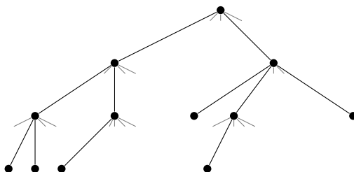
FIGURE 2. The associated 5-ary tree, where each vertex can have children in five different positions (far left, left, middle, right, far right).
