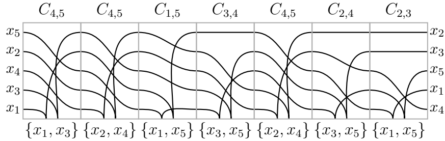
Figure 7: A card sequence for the matrix M
