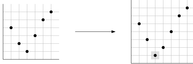
Figure 5: Example of a construction from Case 3. Consider a permutation \pi = 421356 , which has \text{slope}(\pi) = 4 , and suppose we have a pattern \sigma with \text{tail}(\sigma) > 4 . Then f(\pi) = 5312467 .
