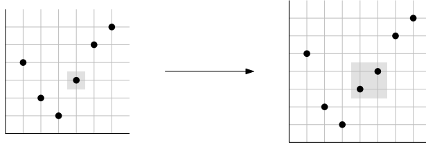
Figure 4: Example of a construction from Case 2. Consider a permutation \pi = 421356 , which has \text{slope}(\pi) = 4 , and suppose we have a pattern \sigma with \text{tail}(\sigma) = 3 . Then f(\pi) = 5213467 .
