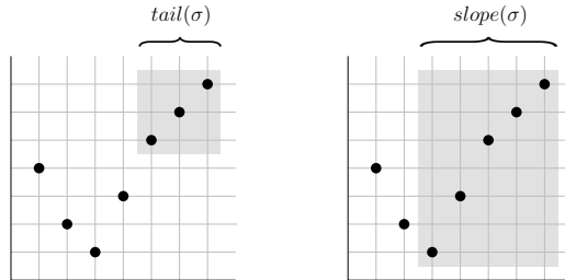
Figure 3: The tail and slope statistics of the permutation \sigma = 4213567
