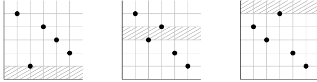
Figure 7: The constructed cores for m = 15 , from left to right for i = 1, 2, 3 . Any permutation with such core and no element in the grey strip is \Pi -avoiding.
