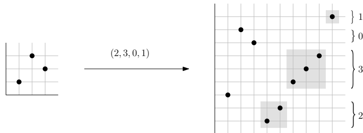
Figure 1: For a permutation \sigma = 132 and 4-tuple a = (2, 3, 0, 1) we have \pi = \sigma \cdot a = 387124569 .
