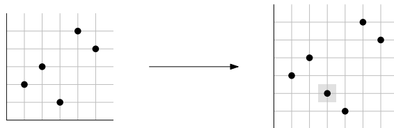
Figure 2: Example of an insertion 23154[3 \rightarrow 2] = 342165
