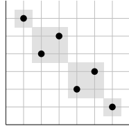
Figure 6: The constructed co-layered permutation for m = 15 and k = 3 . In this case we get d = 4 , s = 1 and p = 1 .
