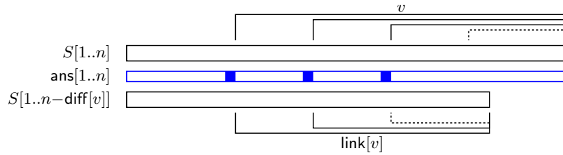
Fig. 2. Series of a palindrome v in S[1..n] and of \text{link}[v] in S[1..n-\text{diff}[v]] . Leading palindromes of the next series are shown by dash lines. The function \text{getMin}(v) returns the minimum of the values of \text{ans} in the marked positions, plus one.
