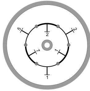
FIGURE 9. Çark corresponding to the class represented by the form (7, 33, -15) . Bold edges are reduced.
