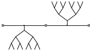
FIGURE 2. The graph of a reciprocal class. Edges of this graph parametrize the reciprocal forms in this class.
