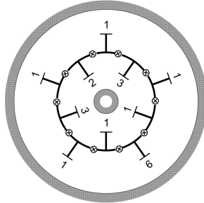
FIGURE 12. Çark corresponding to the ambiguous form f = (3, 18, -11) .
