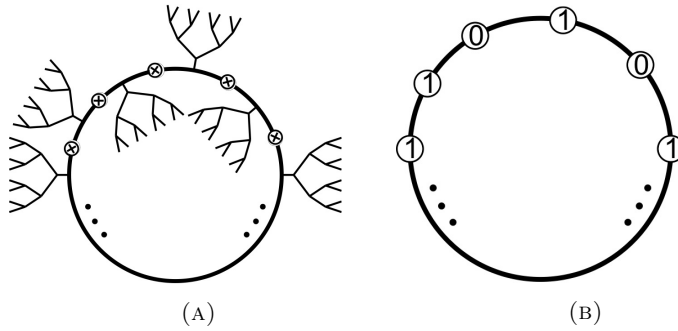
FIGURE 7. From çarks to bracelets
