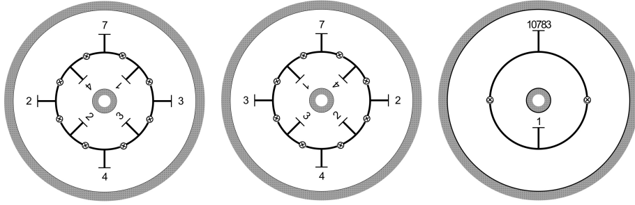
(A) Çark corresponding to f = (-2377, 10173, 1349) . (B) Çark corresponding to f^{-1} = (-4027, 8915, 2287) . (C) Çark of the product of f \times f^{-1} .
