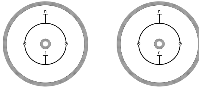
(A) (a) Identity for \Delta = n^2 + 4n . (B) (b) Identity for \Delta = n^2 + 4 .
