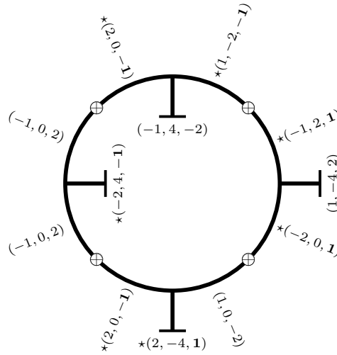
FIGURE 16. Minimum edges of \mathcal{F}/\text{Aut}(\{(1, 0, -2)\}) (* stands for forms which attain the minimum.).
