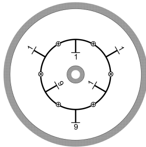
FIGURE 15. Çark corresponding to the reciprocal form f = (-8, 11, 8) .
