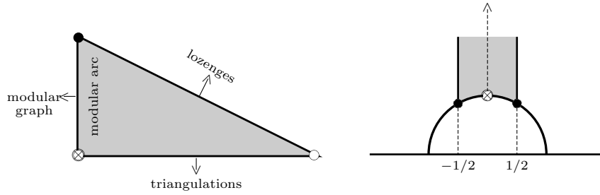
(A) The fundamental region for the modular curve in the upper half plane model. (B) The modular curve. Note that there are two triangles, the second is on the back of the page, glued to this one.
