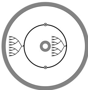
FIGURE 6. The çark \mathcal{F}/\langle SR^2SR \rangle .
