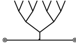
FIGURE 13. The graph \mathcal{F}/\langle S, R^2SR \rangle
