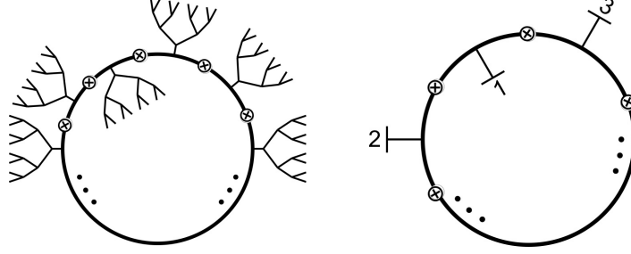
FIGURE 8. A çark and its short form.
