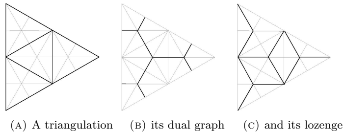
FIGURE 5. Triality of graphs
