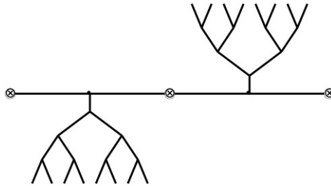
FIGURE 14. The graph \mathcal{F}/\langle RSR^2, S(RSR^2)S \rangle
