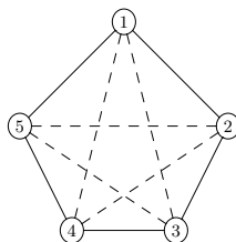
Fig. 1. A R(3, 3; 5) Ramsey graph: edges denoted by solid lines and non-edges by dashed.
