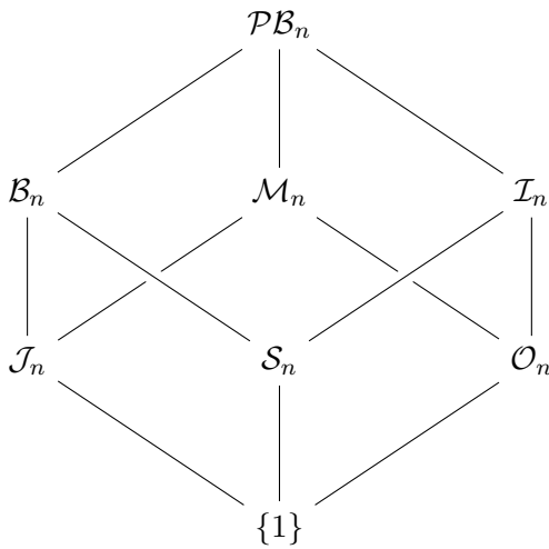
Figure 2: Important submonoids of \mathcal{PB}_n (left) and representative elements from each submonoid (right). See text for further explanation.
