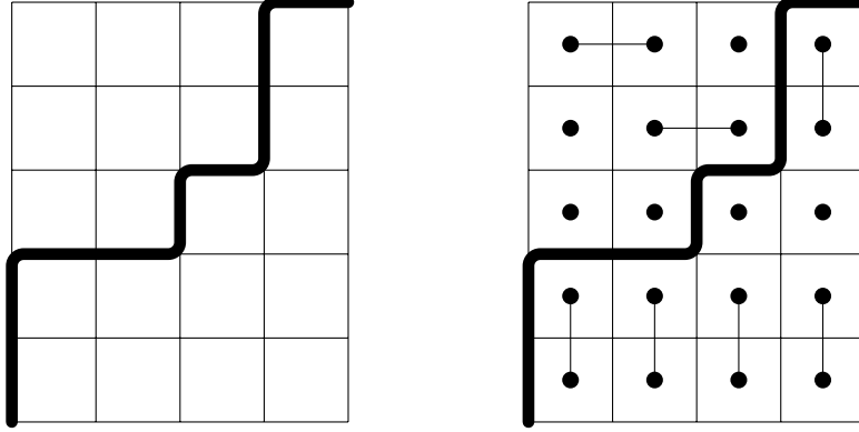
FIGURE 4. The partition \lambda = (3, 3, 2, 0, 0) inside a 5 \times 4 rectangle and a matching of weight s^6 t^7 .
