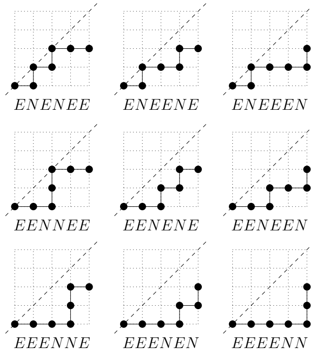
FIGURE 1. Ballot paths of length 6 with 2 North steps.
