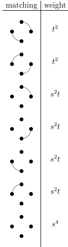
FIGURE 3. The seven Lucas matchings for n = 4 , with corresponding weight.
