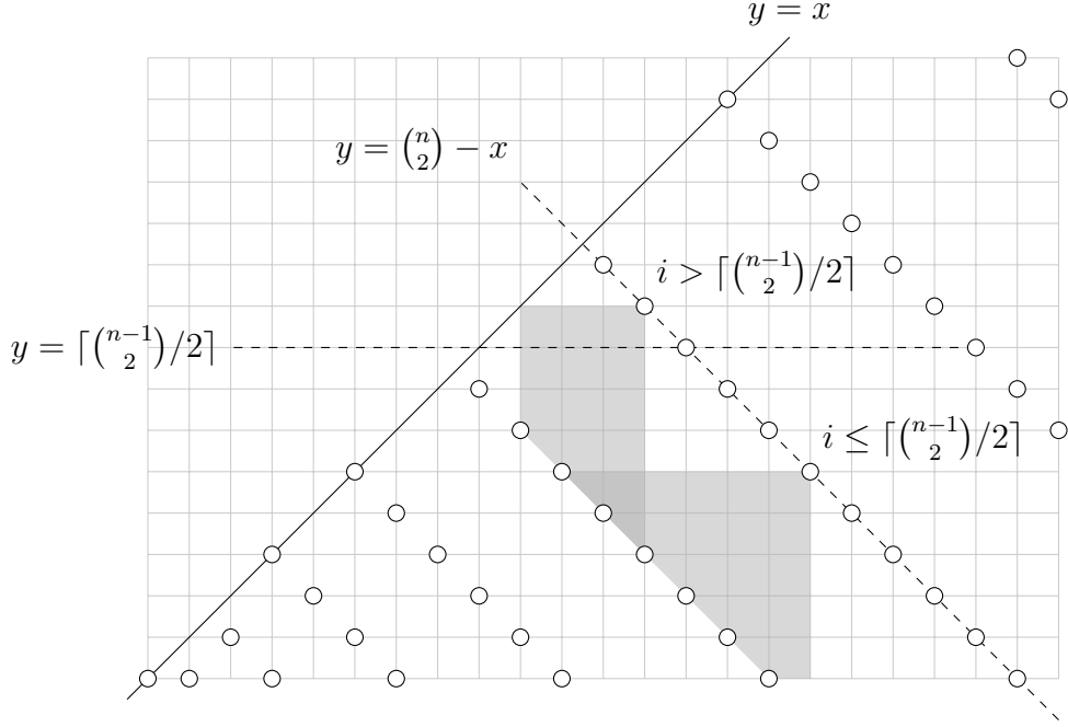
FIGURE 7. The boundary conditions for the recurrence given in Proposition 4.4. Possible locations for anchor nodes are indicated in white.
