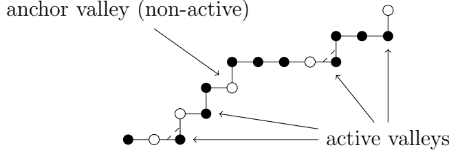
FIGURE 6. A decorated path of length d = 15 .
