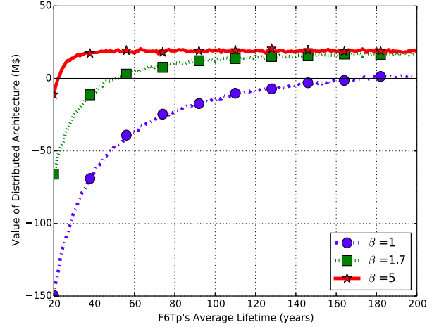
Fig. 6. Effects of F6TPs reliability parameters on value of distributed architecture (i.e., project lifetime=15 years).
