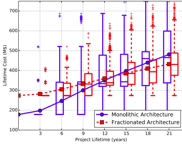
Fig. 4. Total cost of monolithic ( M_2 ) vs. fractionated ( M_3 ) architecture discounted to present time graphed against project lifetime for 10,000 trials. The curves represent expected values, and the boxplots depict quartiles of the cost.
