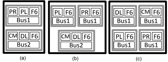
Fig. 7. Allocation of subsystems between fractions together with the number of fractions in Table III, (a) two fractions, (b) three fractions, (c) four fractions (PR: Processor, DL: Downlink, CM: Communication Module, F6: F6TP, PL: Payload)
