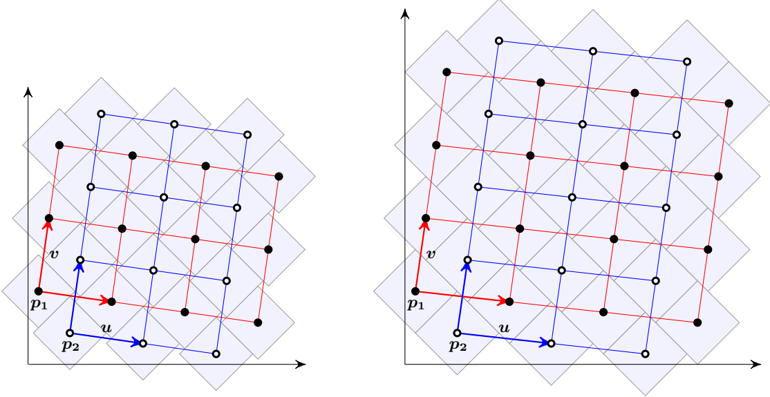
FIGURE 6. Plots of the permutations \sigma_5 \in S_{24} and \sigma_6 \in S_{31} , showing their construction from two interlocking grids of lattice points.
