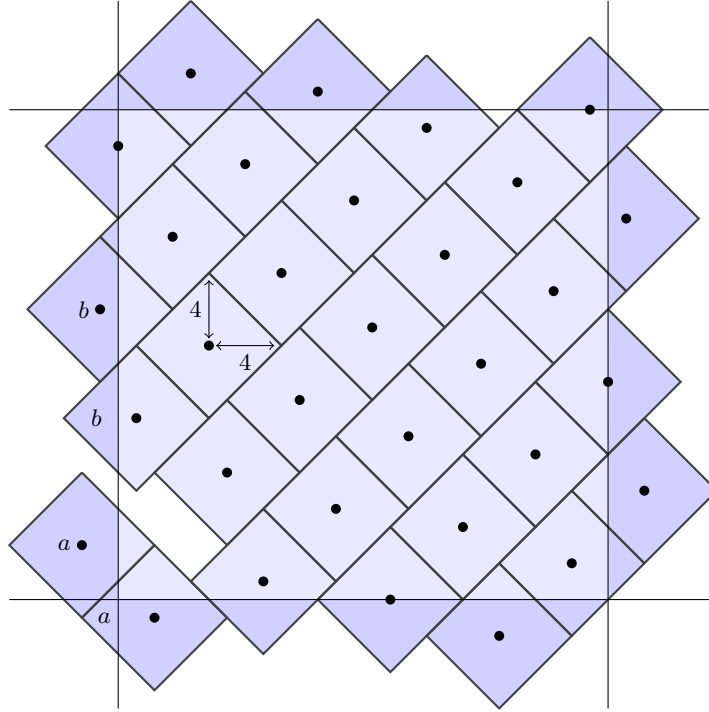
FIGURE 4. The permuted diamond packing corresponding to a 6-prolific permutation, showing the square box used in the proof of Theorem 3.4.
