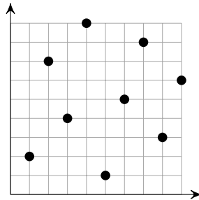
FIGURE 1. The plot of the permutation 274915836.
