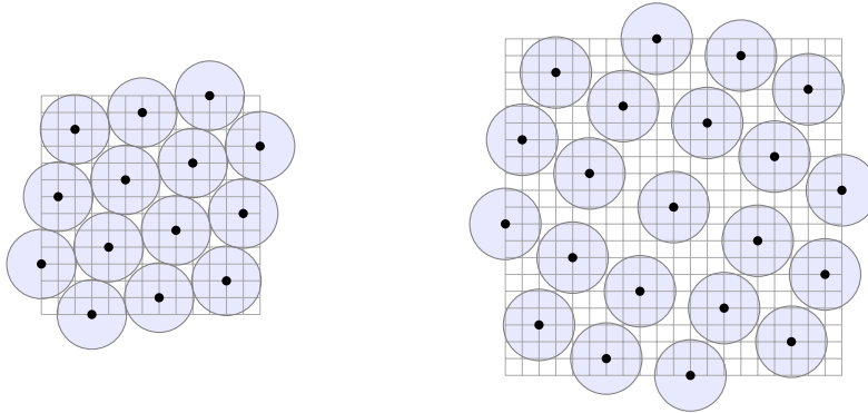
FIGURE 9. Minimal permuted packings of circles of diameter \sqrt{17} and \sqrt{18} + \varepsilon .
