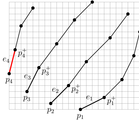
FIGURE 3. An illustration of the second half of the proof of Lemma 2.20, for k = m = 4 .
