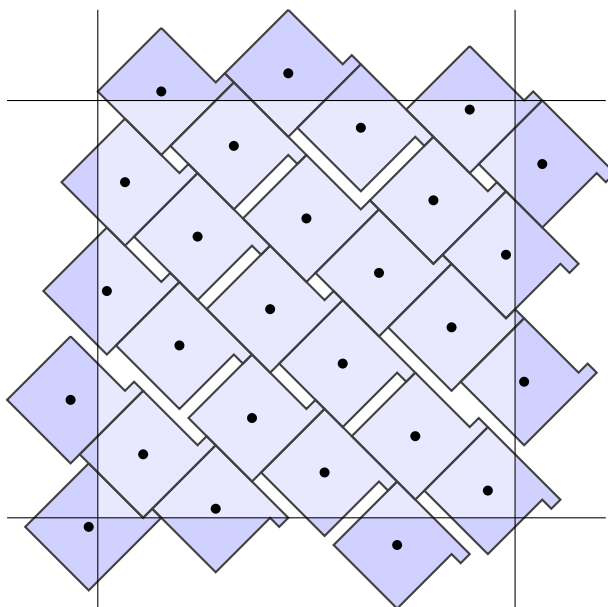
FIGURE 5. A permuted packing of extended diamonds corresponding to a 5-prolific permutation.
