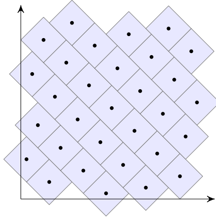
FIGURE 7. An alternative 6-prolific permutation in S_{31} .
