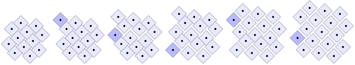
FIGURE 8. Plots of the 3-prolific permutations \sigma_3^{+j} , for j = 0, \dots, 5 ; note that \sigma_3^{+5} is, in fact, 4-prolific.
