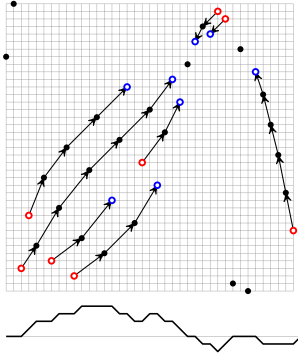
FIGURE 2. An oriented chain graph (Definition 2.3), and a plot of the discrepancy (Definition 2.4) of its vertices. The edges of each chain are oriented away from its red end-vertex towards its blue end-vertex.
