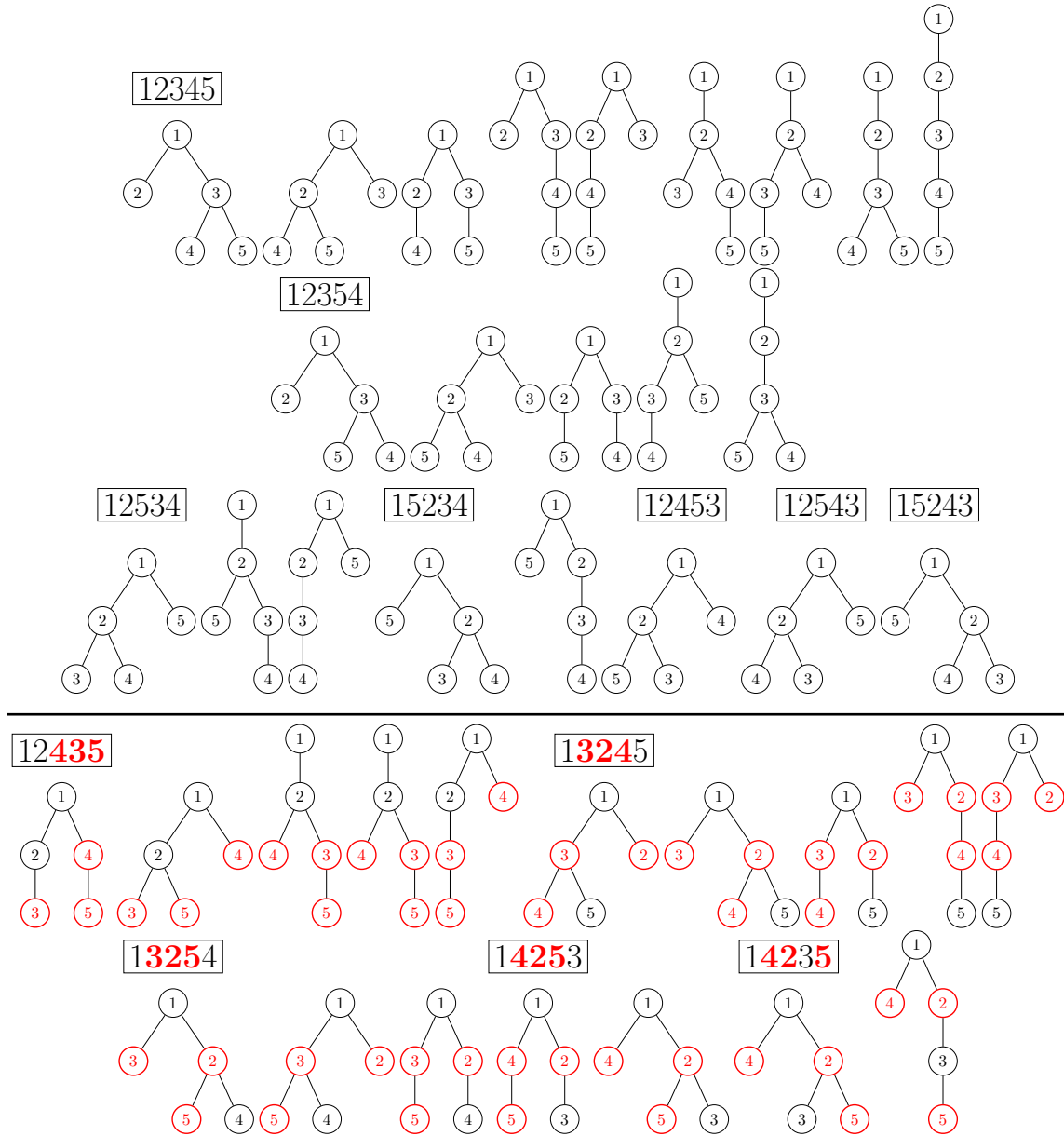
FIGURE 7. All increasing unary-binary trees with 5 nodes, where patterns 213 are marked in red. There are 22 trees (drawn in black) for which the associated permutation avoids this pattern.
