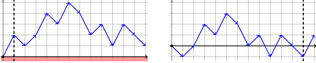
FIGURE 5. Transforming a G_{0,1}(z) instance into a W_{0,1}(z) instance.
