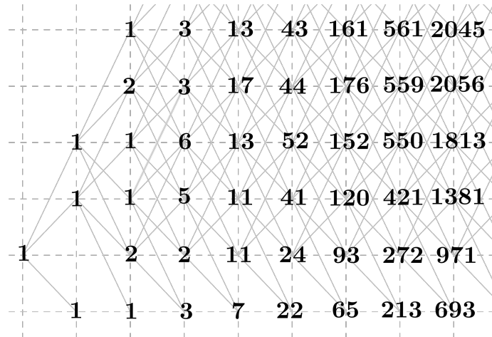
FIGURE 6. Cutting a 4-nomial tree at one unit from its root gives the above picture, which thus naturally corresponds to the lattice supporting our lattice basketball walks. The numbers near each node indicate the number of walks from the root to this node.
