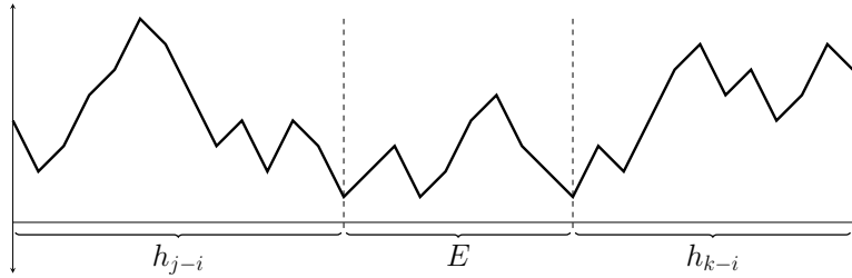
FIGURE 4. The decomposition for G_{j,k}
