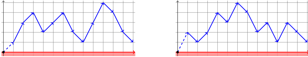
FIGURE 3. Two different instances of walks counted by G_{0,1}(z) showing the two possible first steps +1 and +2 .
