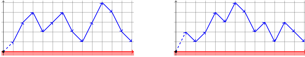
FIGURE 3. Two different instances of walks counted by G_{0,1}(z) showing the two possible first steps +1 and +2 .
