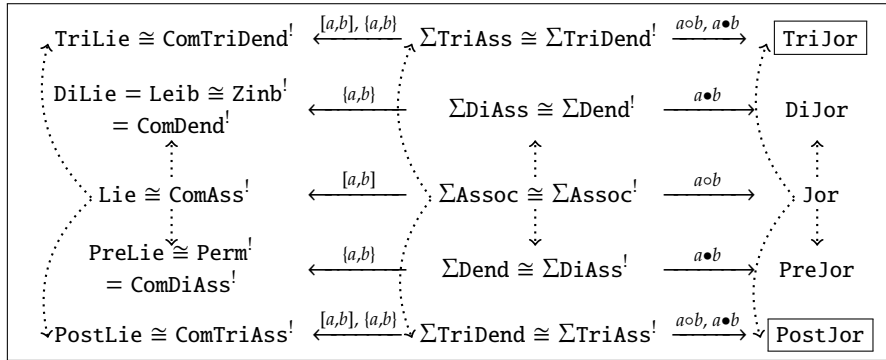
FIGURE 1. Generalizations of the Lie, associative, and Jordan operads
