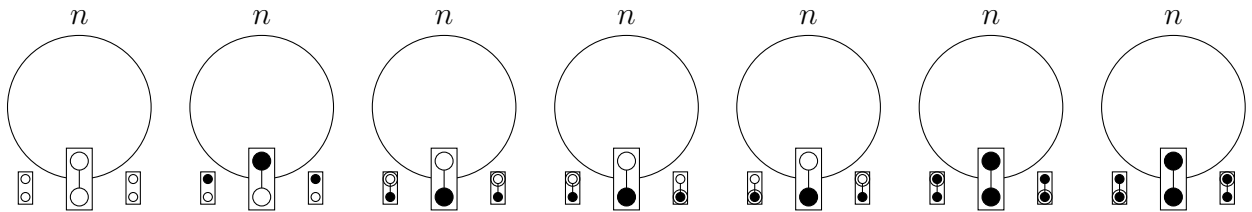
FIGURE 16. A circular raft, and all seven legal labelings.
