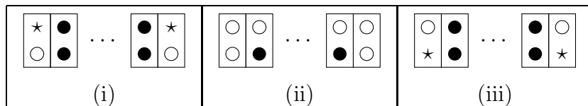
FIGURE 9. Patterns that are forbidden for lex-minimal presentations.
