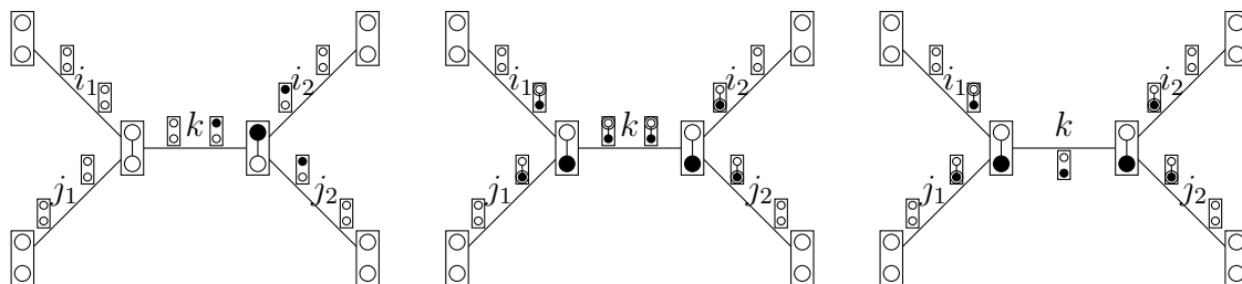
FIGURE 17. A harbor graph with two wharfs and some of its legal labelings.
