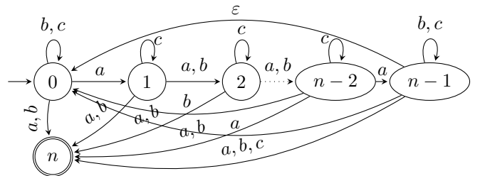
Fig. 4. An NFA \mathcal{B}_n marking language g(h^{-1}h(\bigcup_{a \in \Sigma} (\overline{K}_n/a)a') \cap \Sigma^* \Sigma')
