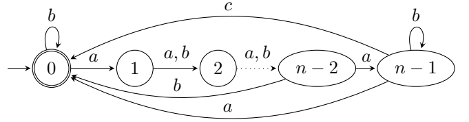
Fig. 3. The minimal DFA \mathcal{A}_n for K_n
