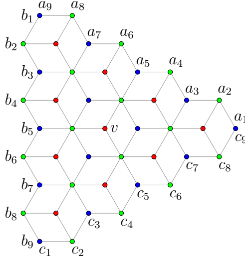
FIGURE 8. The graph G(v, t) for t = 5 .
