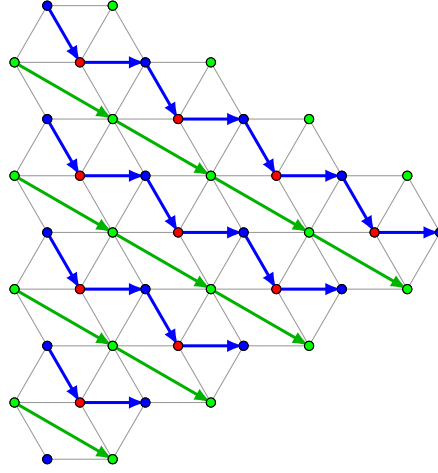
FIGURE 13. The rooted G(v, t) -forest that corresponds to the boundary 0-path in \tilde{N}_{(v, t)} .
