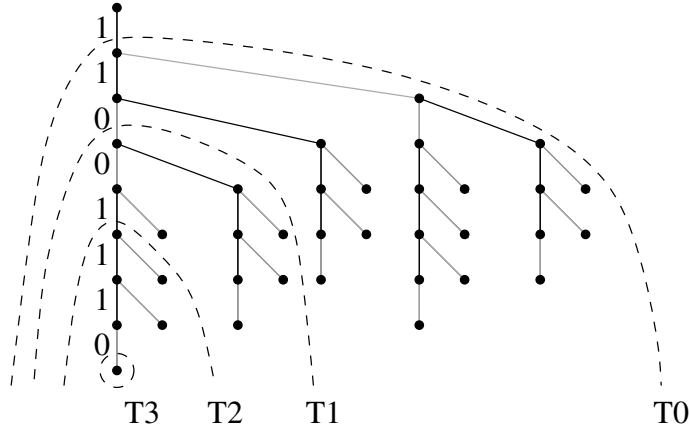
FIGURE 3. The trie \mathcal{T}_{L_2}(11001110) .
