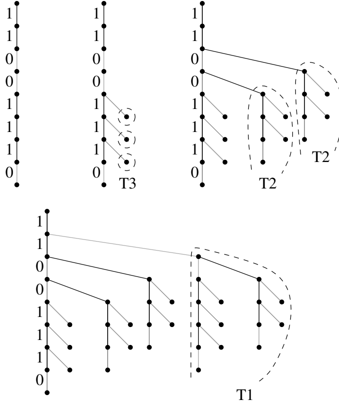
FIGURE 4. Bottom-up construction of \mathcal{T}_{L_2}(11001110) .
