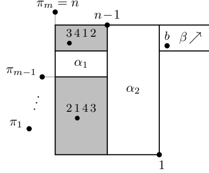
FIGURE 1. A T -avoider counted by J_m with n - 1 before 1
