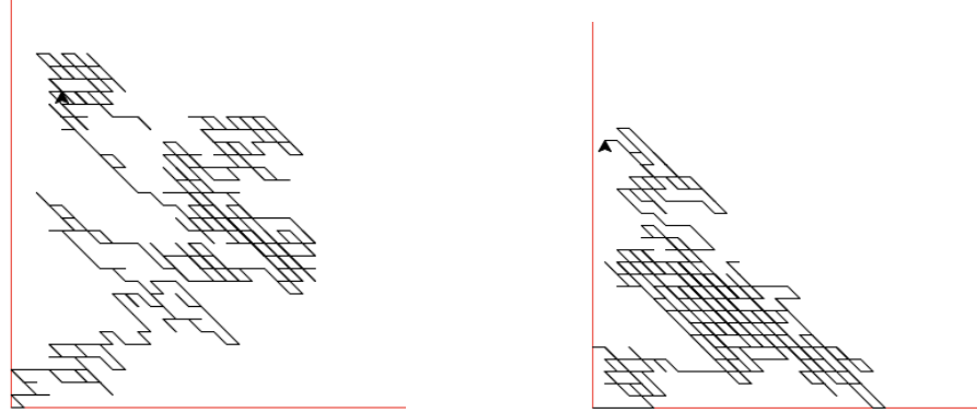
Figure 11.3: Two uniformly sampled Gouyou-Beauchamps walks on 800 steps: an unweighted (balanced) model (left) and a weighted (reluctant) model with parameters a = \frac{1}{\sqrt{2}} and b = 1 (right), which can be scaled to a model with step weights of 1 and 2 by uniformly multiplying each weight by \sqrt{2} .
